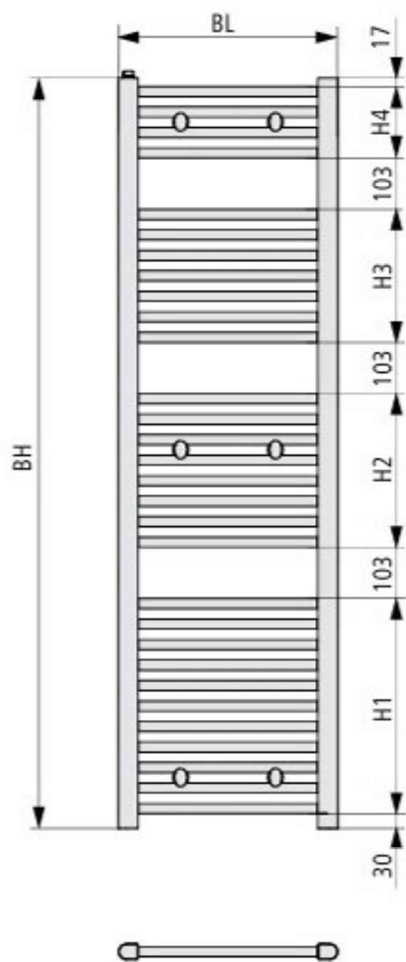
Front view
