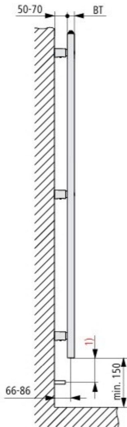
Side view
